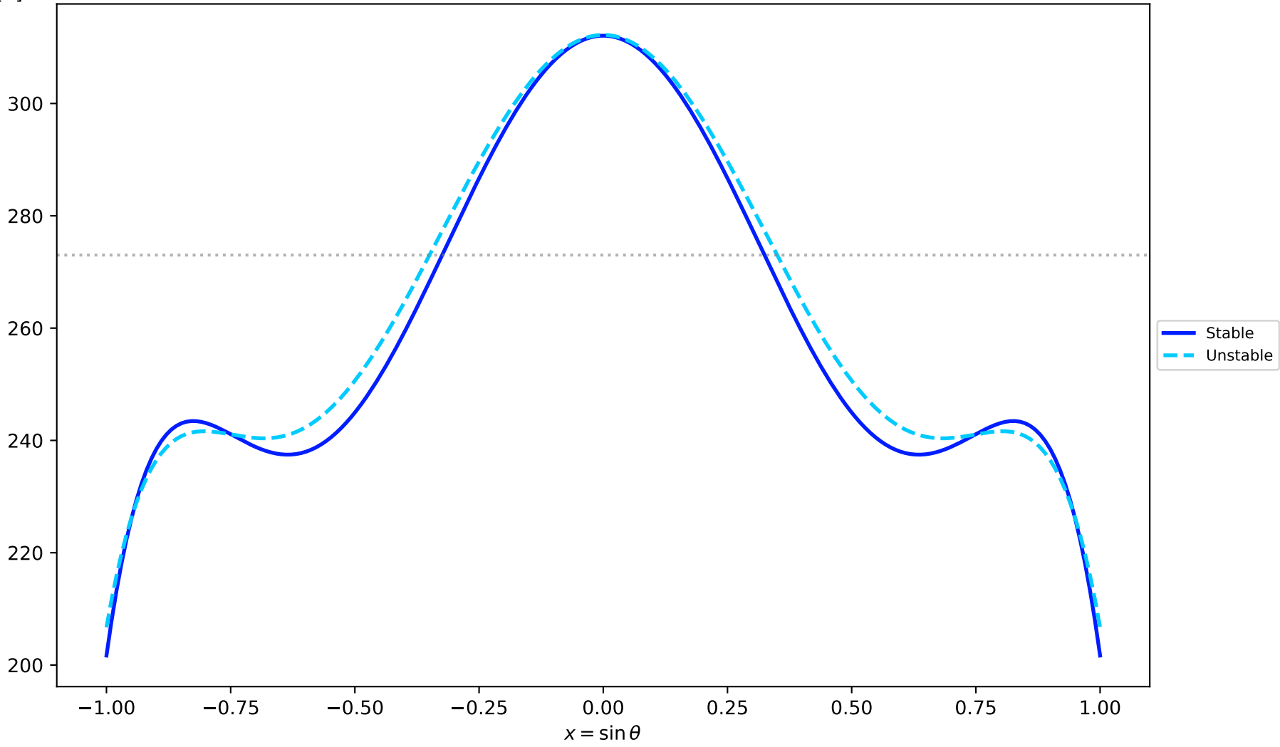
T(x) [K] Temperature Profile around \mu = 30 \text{ W/m}^2
